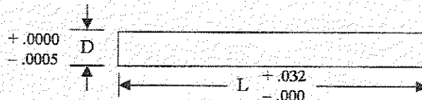
D \times L Straight Pin (Style #1)
