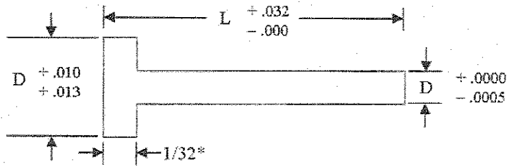
D \times L Headed Pin (Style #2)
