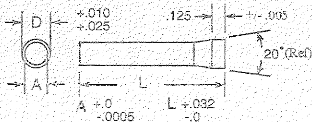
A \times L Style #3
